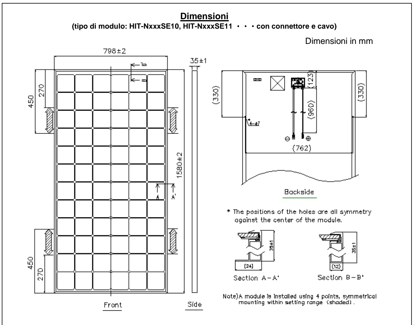
Figure 2-1: Dimensions
