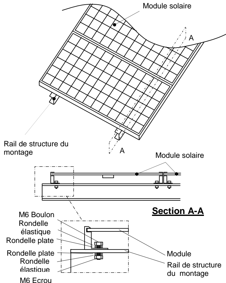
Figure 1: Installation
