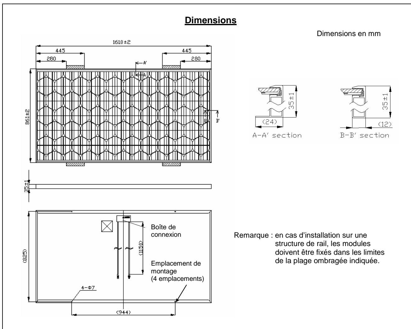
Figure 2-1: Dimensions
