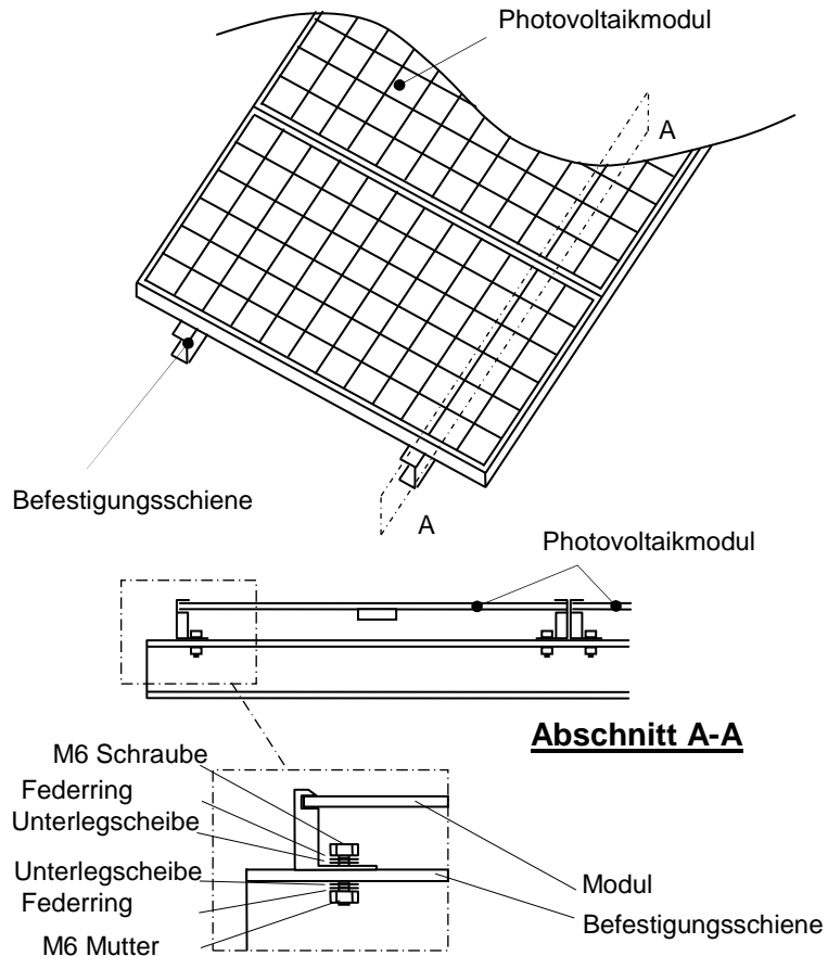
Abb. 1: Installation
